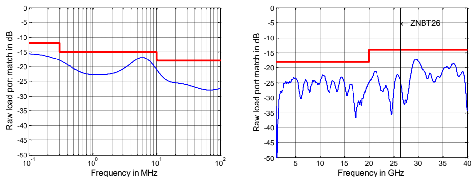
Raw load port match versus frequency for the R&amp;S®ZNBT26/R&amp;S®ZNBT40
